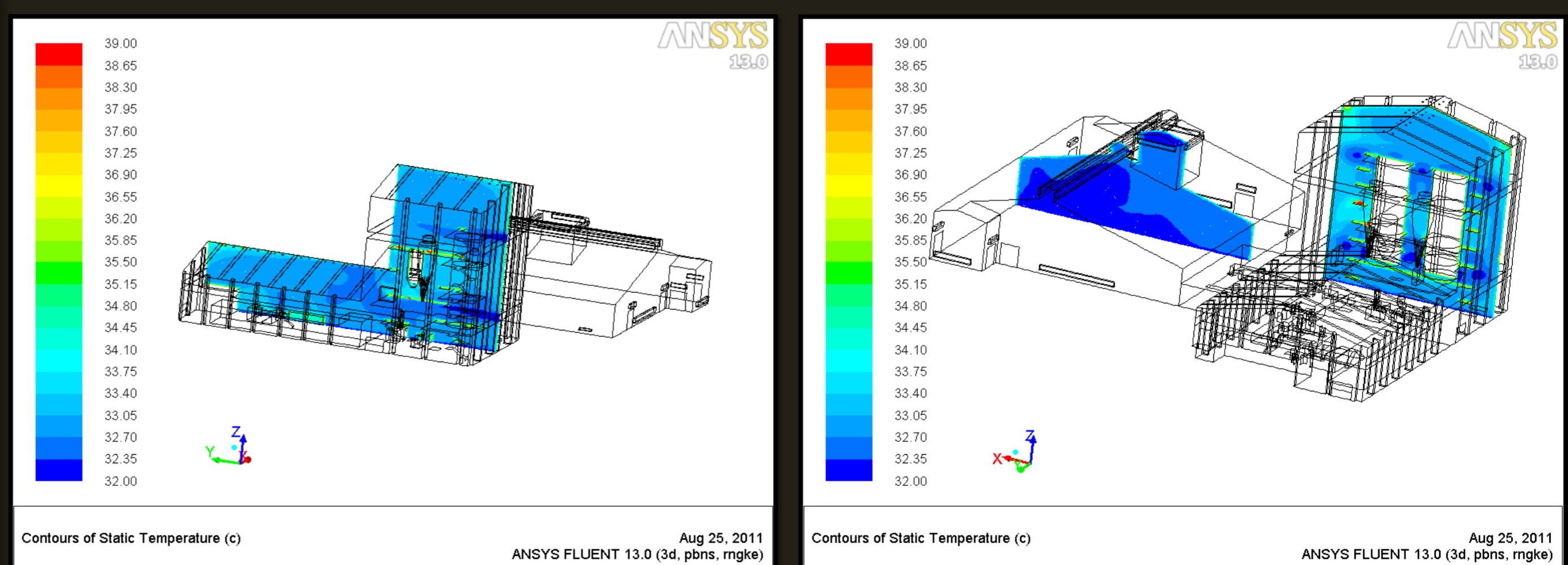
Fig. 3: Temperature Contour along Longitudinal Vertical Plane (Modified Configuration)
